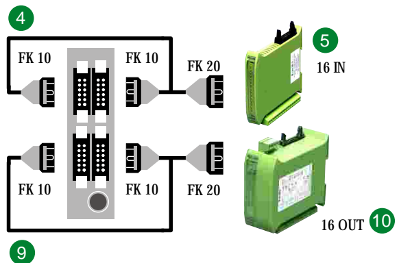
C32T - E32T 16 IN + 16 OUT
